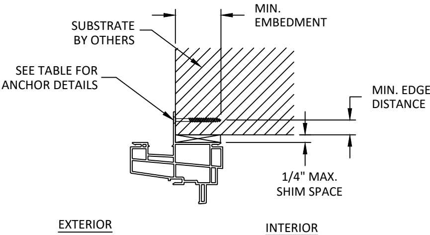
A 5 VERTICAL SECTION HEAD - NAIL FIN NOTE: JAMB & SILL SIMILAR
